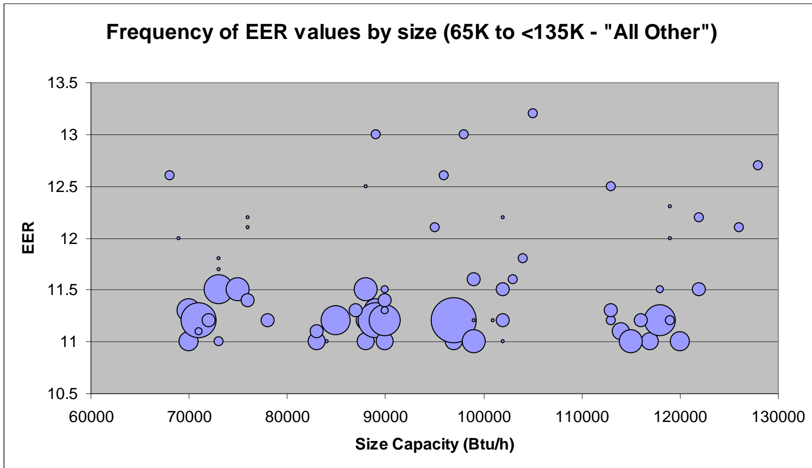
Chart 2. Frequency of EER values by size (65,000 Btu/h to <135,000 Btu/h) – “All Other” Heating Section Type
