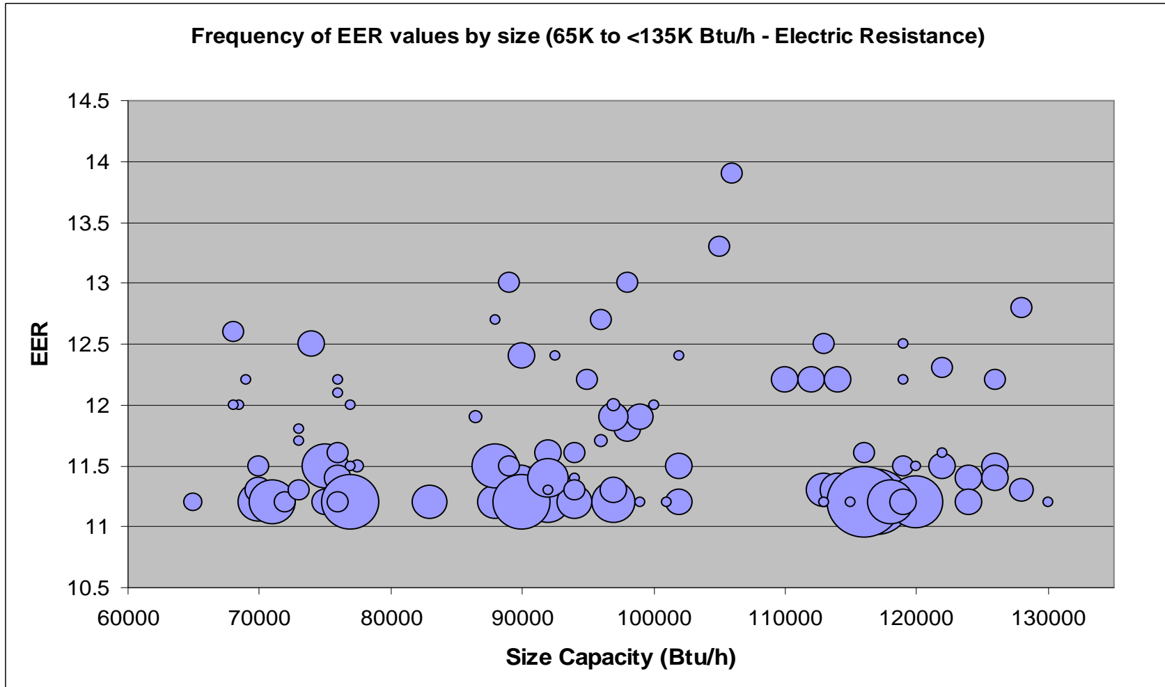
Chart 1. Frequency of EER values by size (65,000 Btu/h to <135,000 Btu/h) – Electric Resistance Heating Section Type
