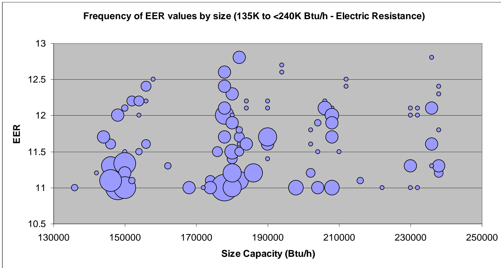
Chart 3. Frequency of EER values by size (135,000 Btu/h to <240,000 Btu/h) – Electric Resistance Heating Section Type
