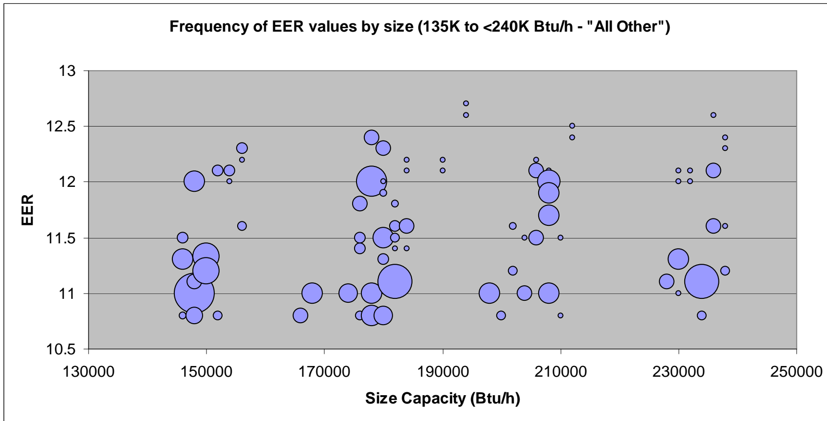
Chart 4. Frequency of EER values by size (135,000 Btu/h to <240,000 Btu/h) – “All Other” Heating Section Type
