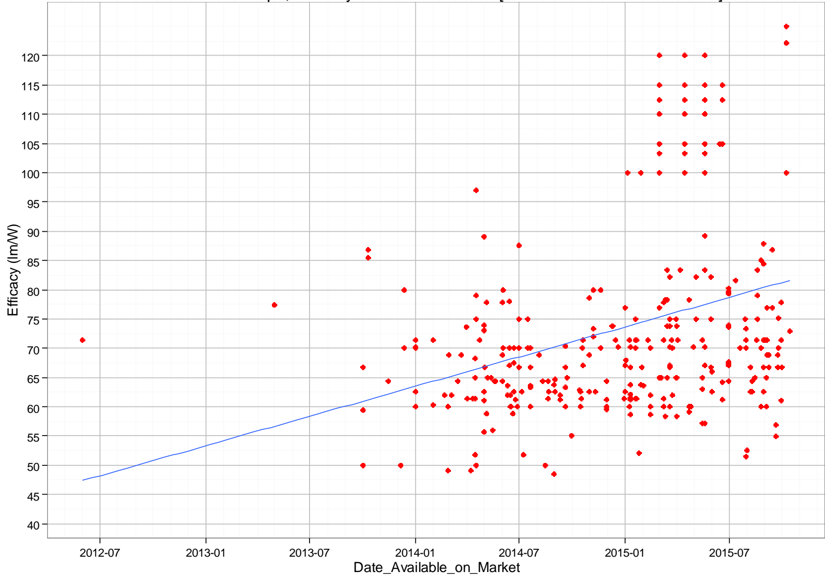
Decorative Lamps, Efficacy vs. Date on Market [698 ENERGY STAR LAMPS]
