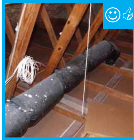
Duct is located in unconditioned space and is properly insulated.
