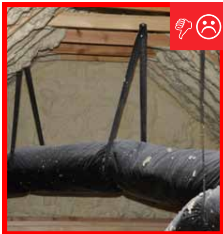
C. Straps are spaced too far apart causing the straps to compress the duct under its own weight.
