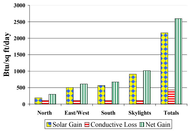
Figure 5f. July 21, double glazing, gas fill, SHGC = 0.38 (South 0.72), U = 0.3; gain = 2,594 Btu/sq ft/day
